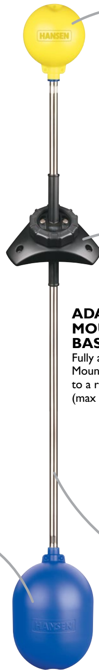
LONG BOTTOM FLOAT 155 x 230mm long bottom float ensures excellent buoyancy for accurate indication of fluid level
